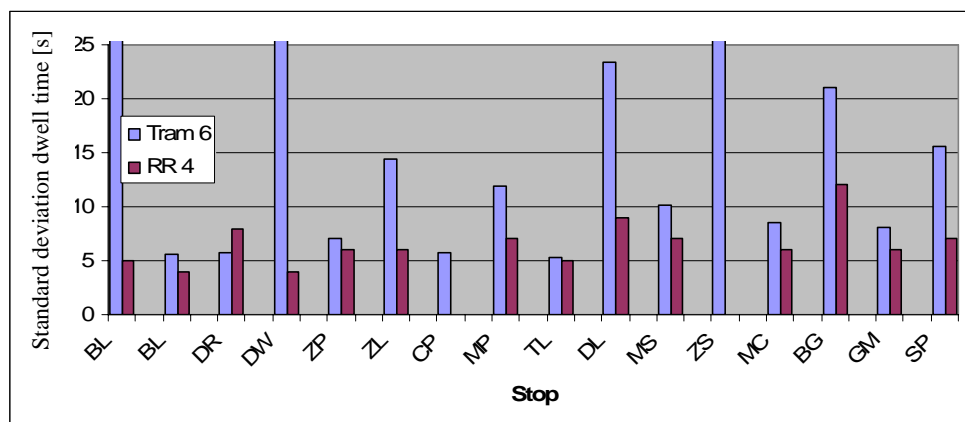
FIGURE 5 Standard Deviations of Dwell Times per Stop before and after the introduction of RandstadRail
