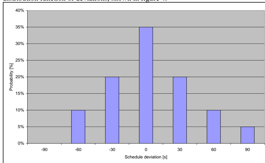
FIGURE 4 Variability in Arrival Time Deviations.
