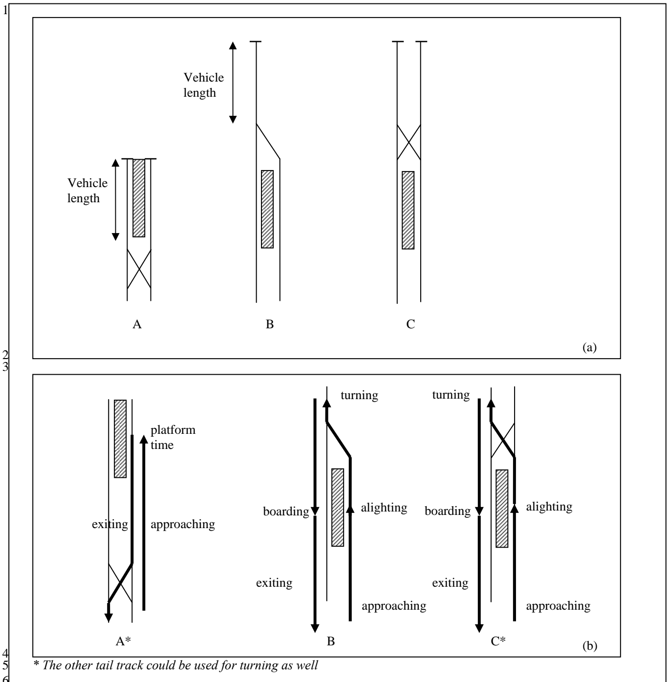
FIGURE 2 Three commonly used Terminal Types (a) and Processes (b).
