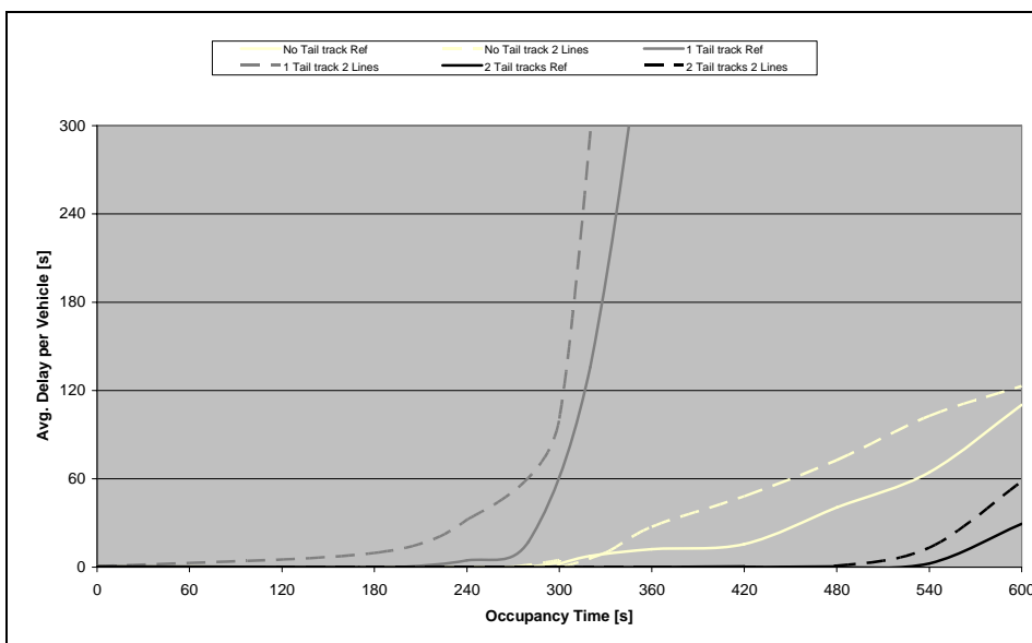
16 17 FIGURE 10 Effects of Number of Lines at Terminals on Average Delay per Vehicle, Total Frequency of 18 12 veh/hour.
