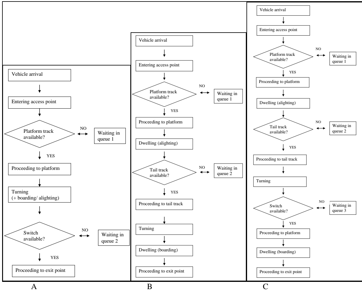
21 22 FIGURE 3 Simulation Steps for Three Terminal Types (A= No Tail Tracks, B= 1 Tail Track and C= 2 23 Tail Tracks). 24 25 26 27
