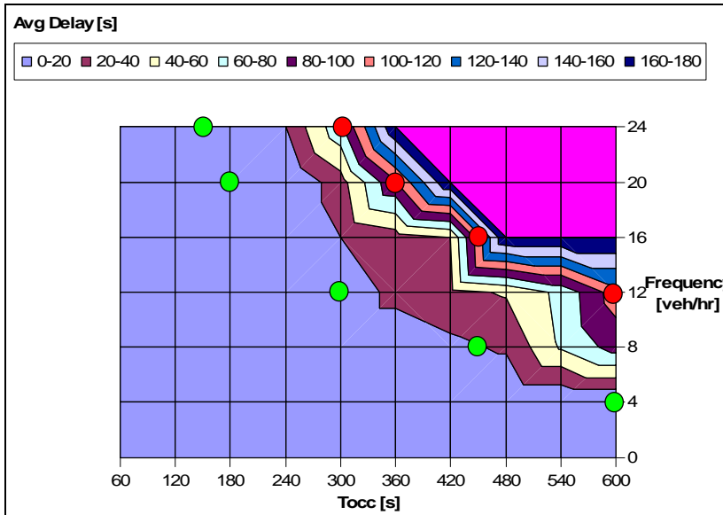
1 2 FIGURE 5 Average Delay as a Function of Occupancy Time and Service Frequency, no Tail Tracks.
