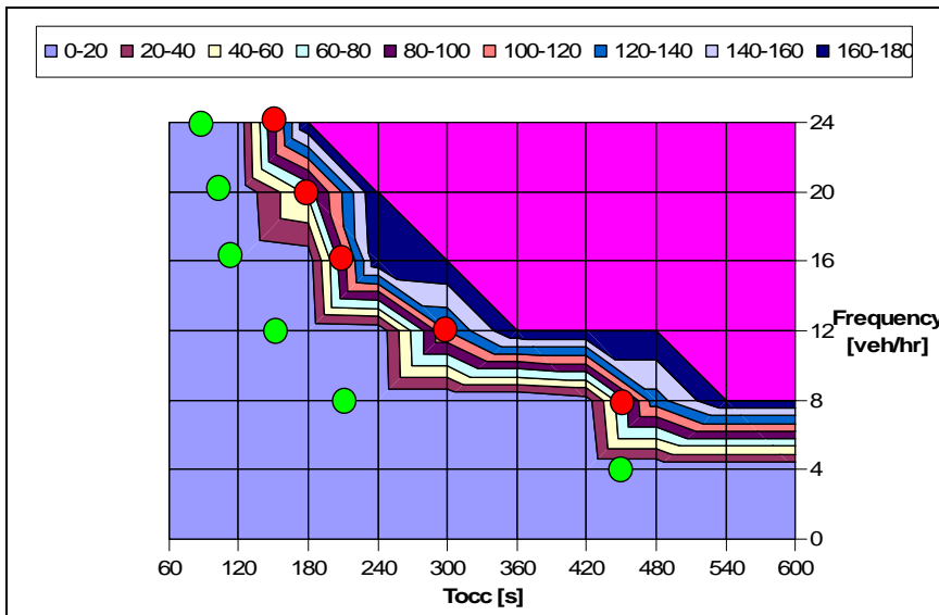
10 11 FIGURE 6 Average Delay as a Function of Occupancy Time and Service Frequency, one Tail Track.
