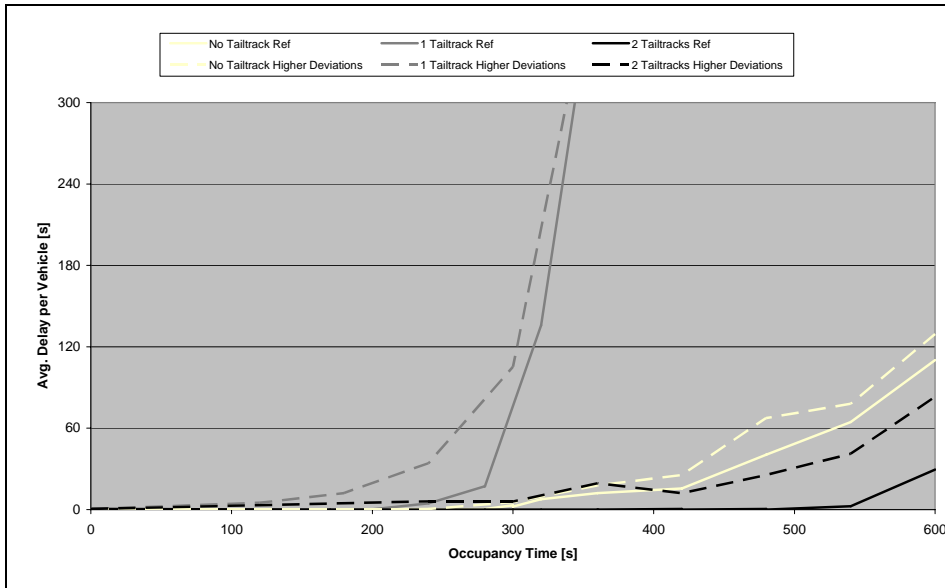
1 2 FIGURE 9 Effects of Schedule Deviations on Average Delay per Vehicle at Terminals.
