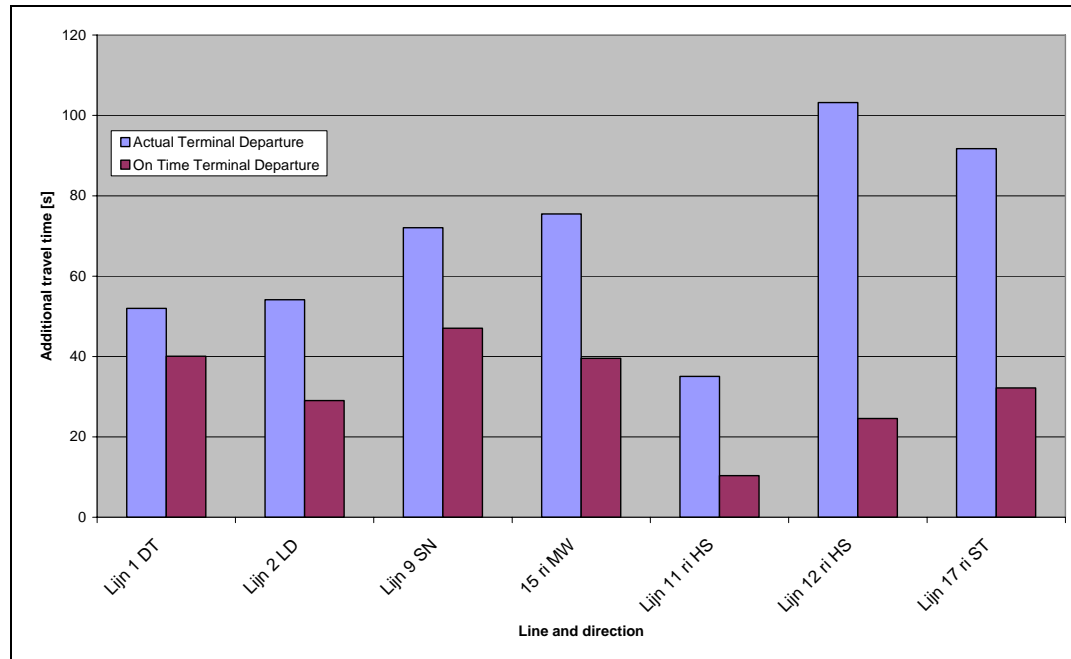
14 FIGURE 1 Effect of on Time Departure at Terminal on Additional Travel Time per Passenger.
