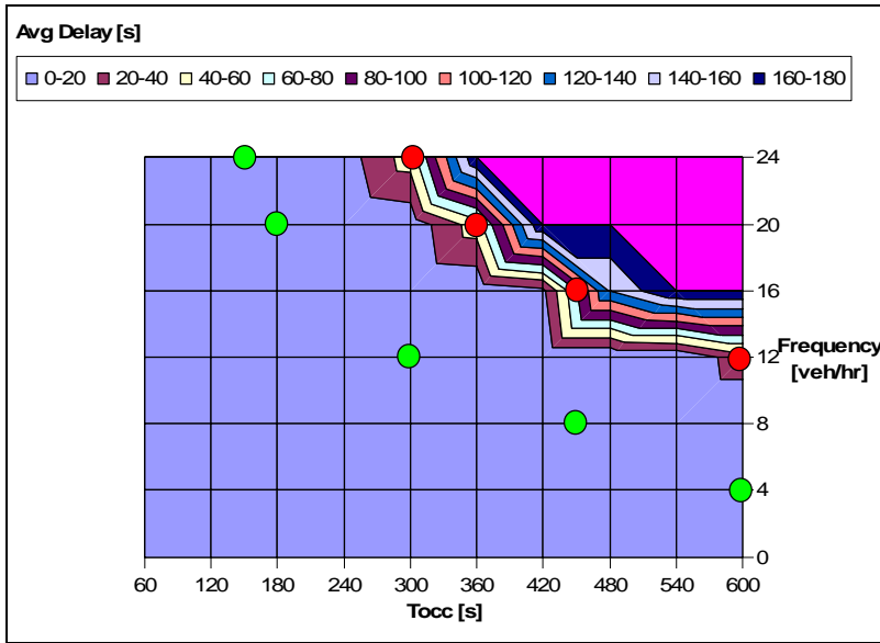
1 2 FIGURE 7 Average Delay as a Function of Occupancy Time and Service Frequency, two Tail Tracks.
