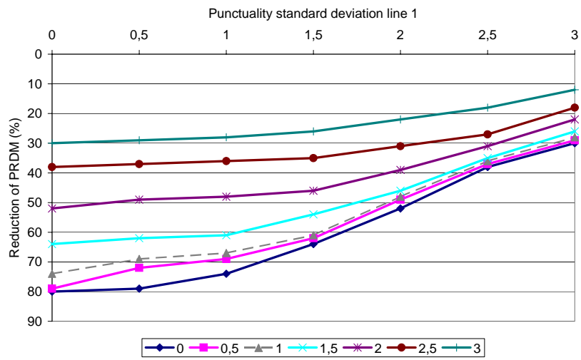
Figure 8: Reduction of the PRDM as a function of the punctuality of line 1 for different values of the punctuality of line 2 due to coordinating the transport services and improving the punctuality by reducing the standard deviation by 1 minute for both lines
