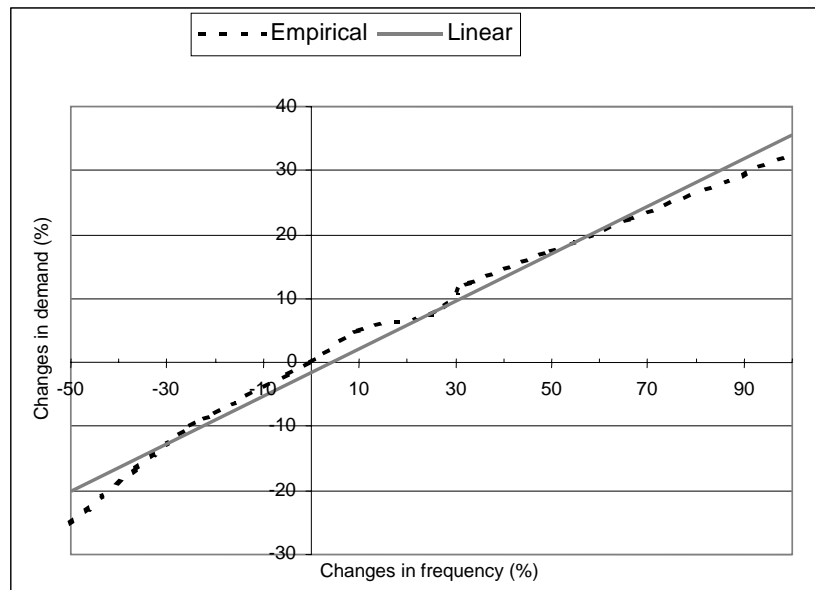
Figure 2: Relationship between changes in frequency and changes in demand (2)
